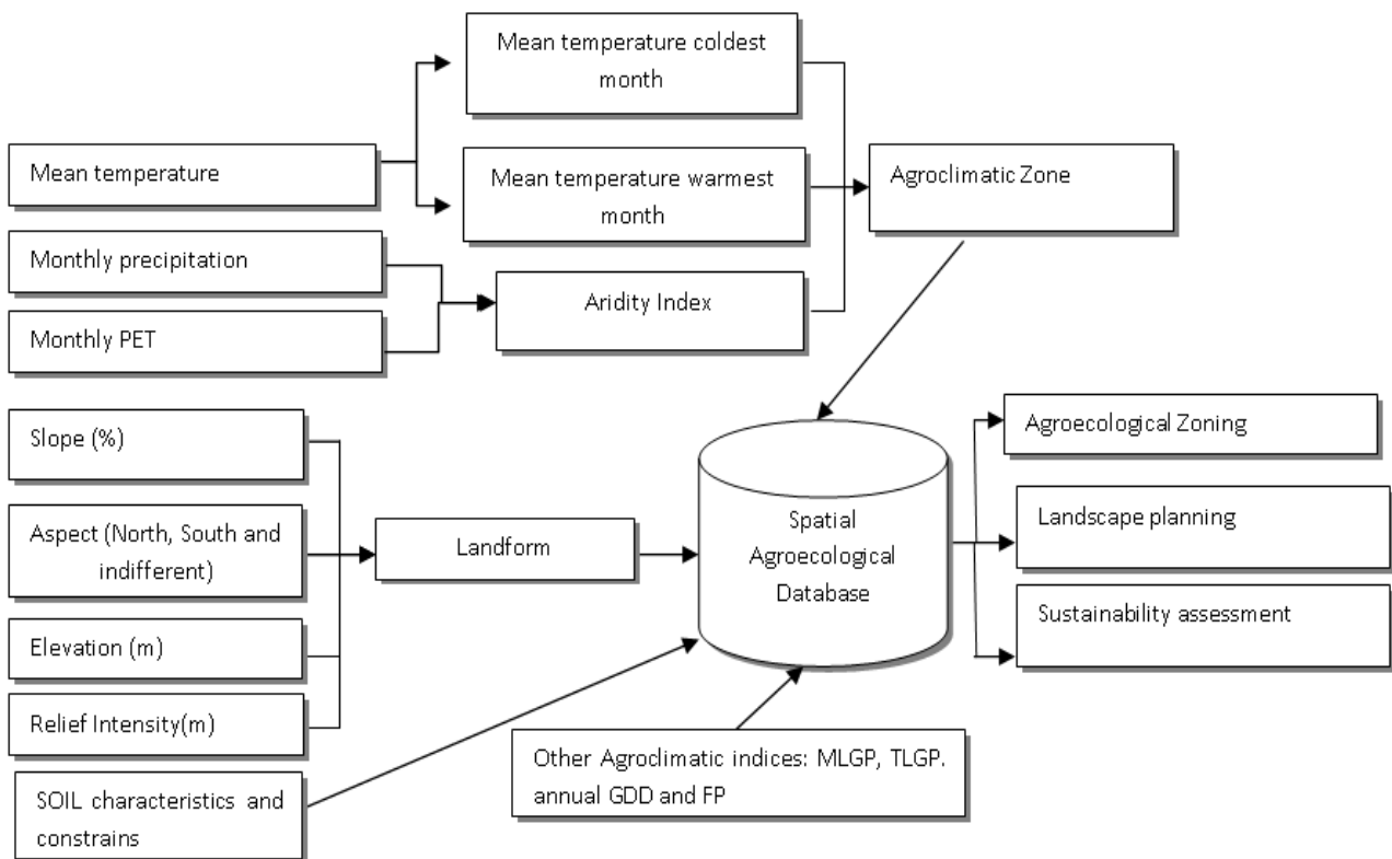
Fig. 2. Framework and information flow for create spatial database and agroecological zoning
